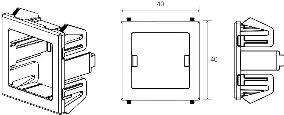
Panel Bracket
