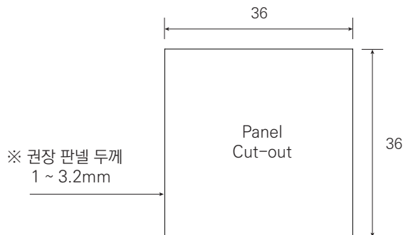
Panel cut-out
