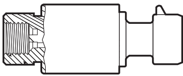
Pressure Port : 7/16-20UNF (female)
